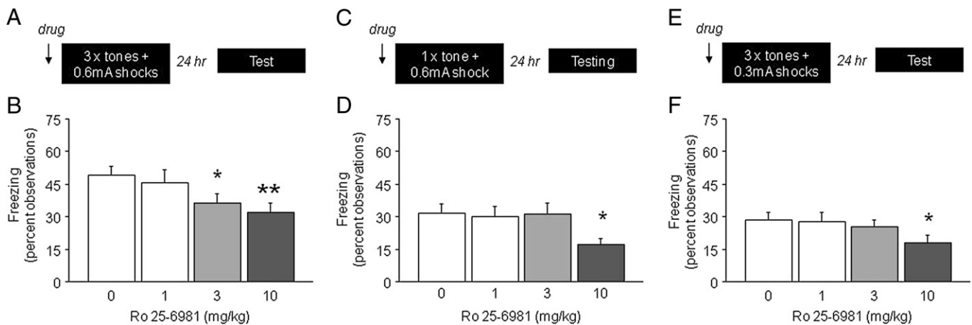
Fig. 1. Fear memory impairing effects of Ro 25-6981 on multi-trial, one-trial and low-lock shock fear conditioning. (A) Schematic of the multi-trial high shock protocol. (B) Pre-training treatment with 10 mg/kg Ro 25-6981 reduced fear recall relative to vehicle (0) ( n=16-18/\text{dose} ). (C) Schematic of the one-trial high-shock conditioning protocol. (D) Pre-training treatment with 10 mg/kg Ro 25-6981 reduced fear recall relative to vehicle (0) ( n=13-14/\text{dose} ). (E) Schematic of multi-trial low-shock protocol. (F) Pre-training treatment with 10 mg/kg Ro 25-6981 reduced fear recall relative to vehicle (0) ( n=15-16/\text{dose} ). ** p<.01 , * p<.05 vs. vehicle (0). Data in Figs. 1–4 are Means \pm SEM.
